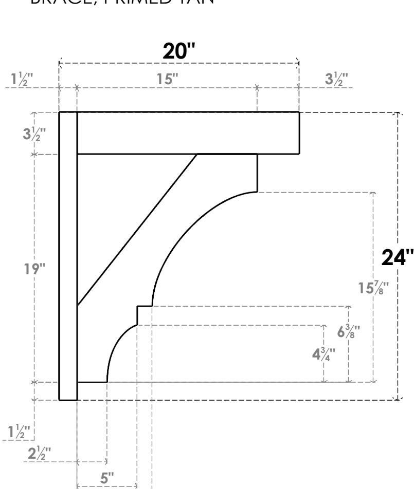
SIDE PROFILE
